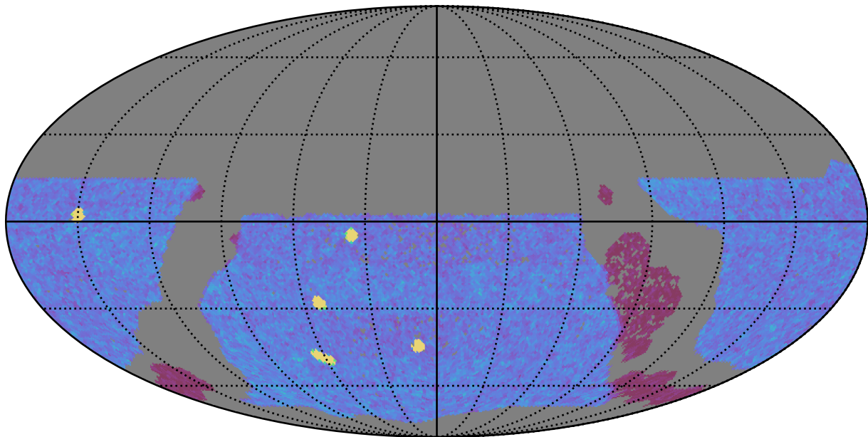
too_elab_r8_d3_gz_v3.4_10yrs WFD y band: NVisits
