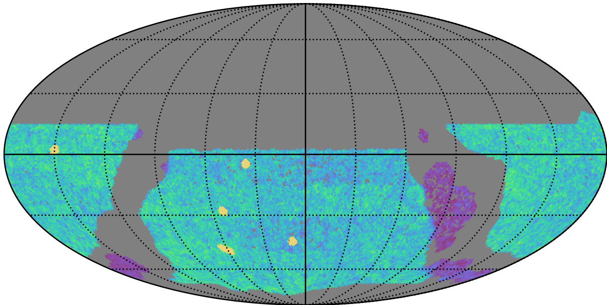
too_elab_r8_d3_gz_v3.4_10yrs WFD u band: NVisits
