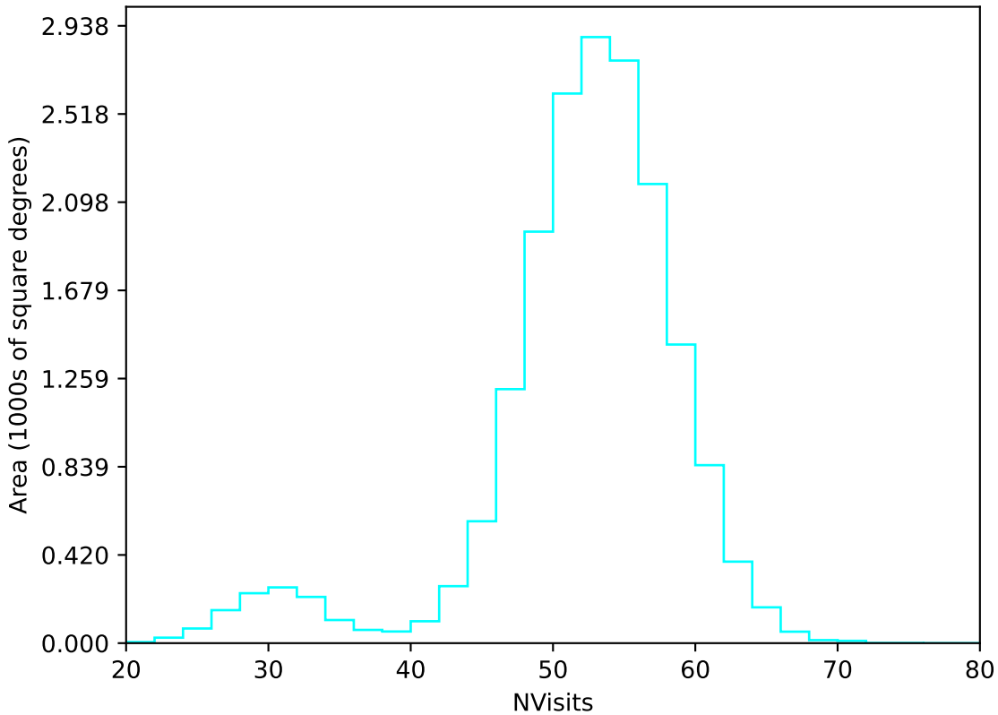
too_elab_r8_d3_gz_v3.4_10yrs WFD u band: NVisits
