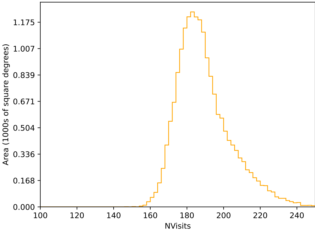
too_elab_r8_d3_gz_v3.4_10yrs WFD r band: NVisits
