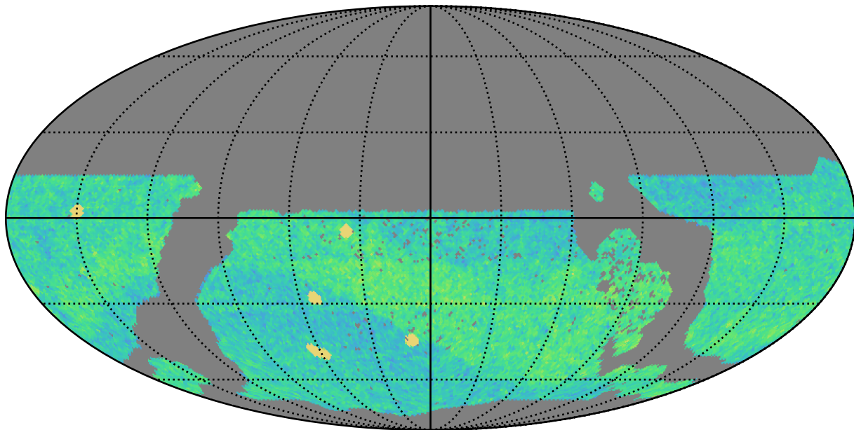
too_elab_r8_d3_gz_v3.4_10yrs WFD i band: NVisits
