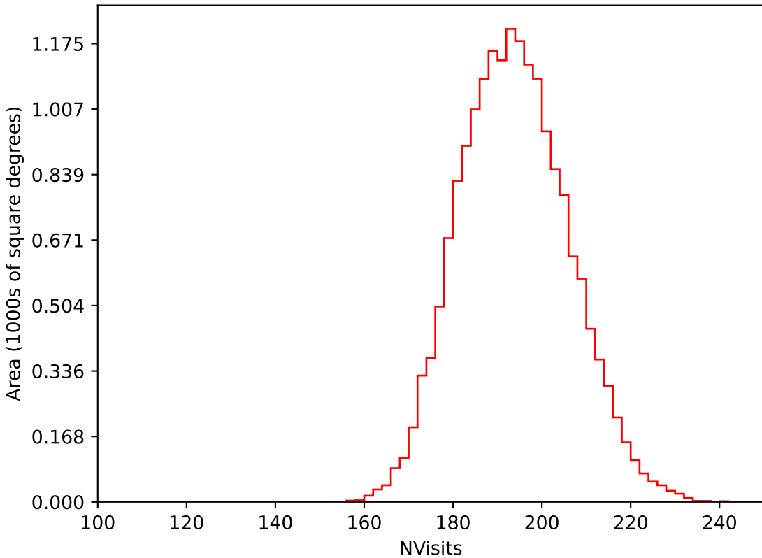
too_elab_r8_d3_gz_v3.4_10yrs WFD i band: NVisits
