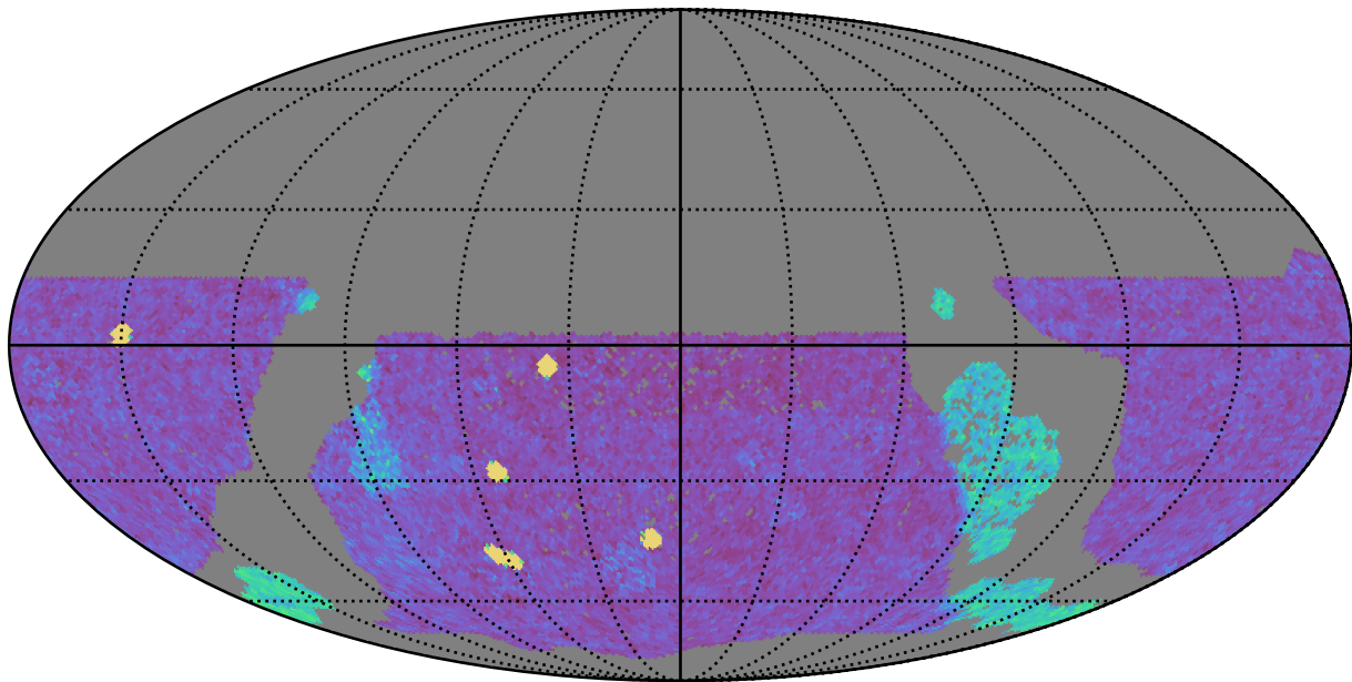
too_elab_r8_d3_gz_v3.4_10yrs WFD g band: NVisits
