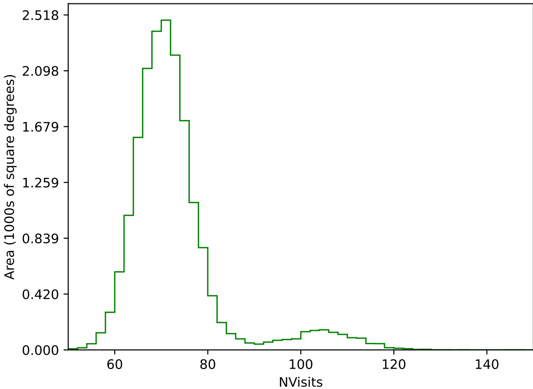
too_elab_r8_d3_gz_v3.4_10yrs WFD g band: NVisits
