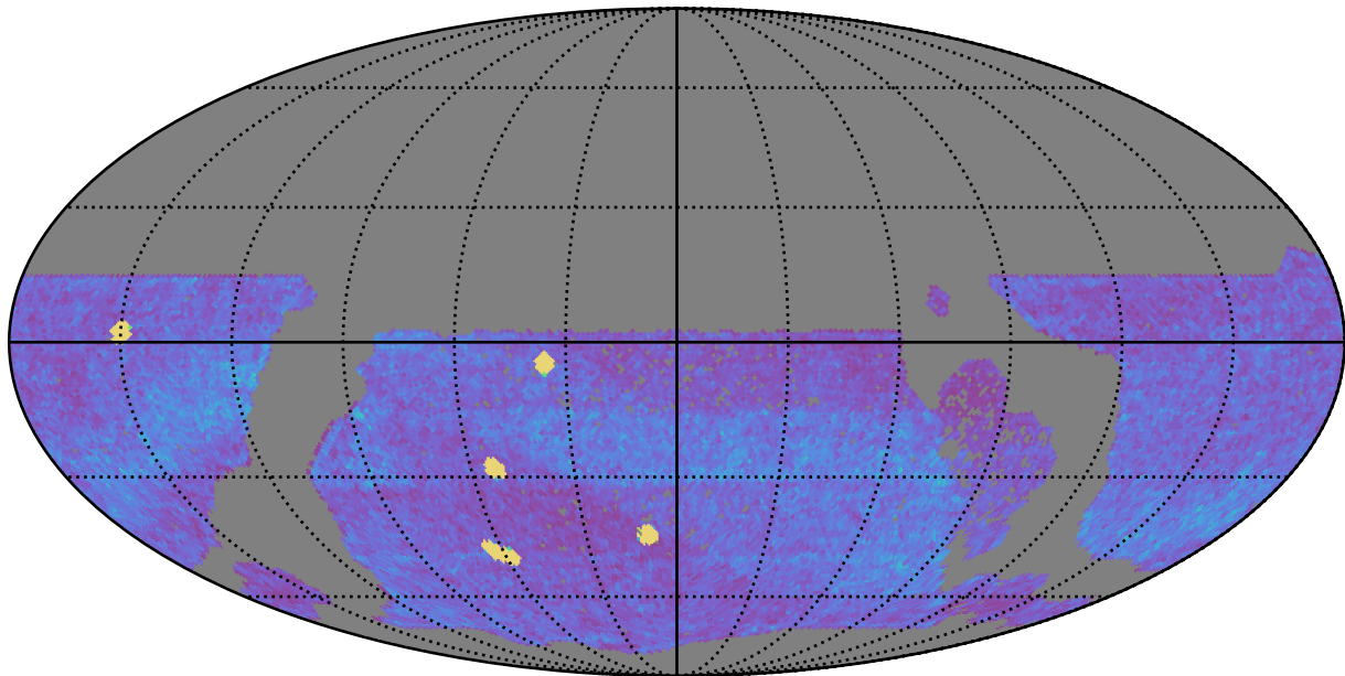
too_elab_r8_d3_gz_v3.4_10yrs WFD all bands: NVisits
