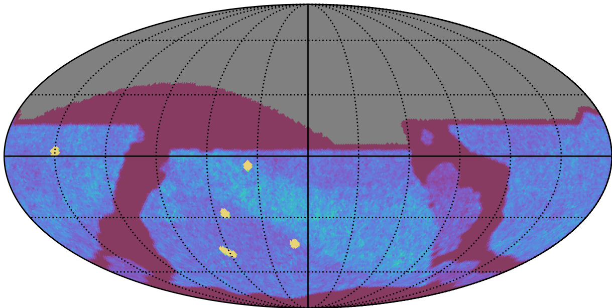
too_elab_r8_d3_gz_v3.4_10yrs All sky z band: NVisits
