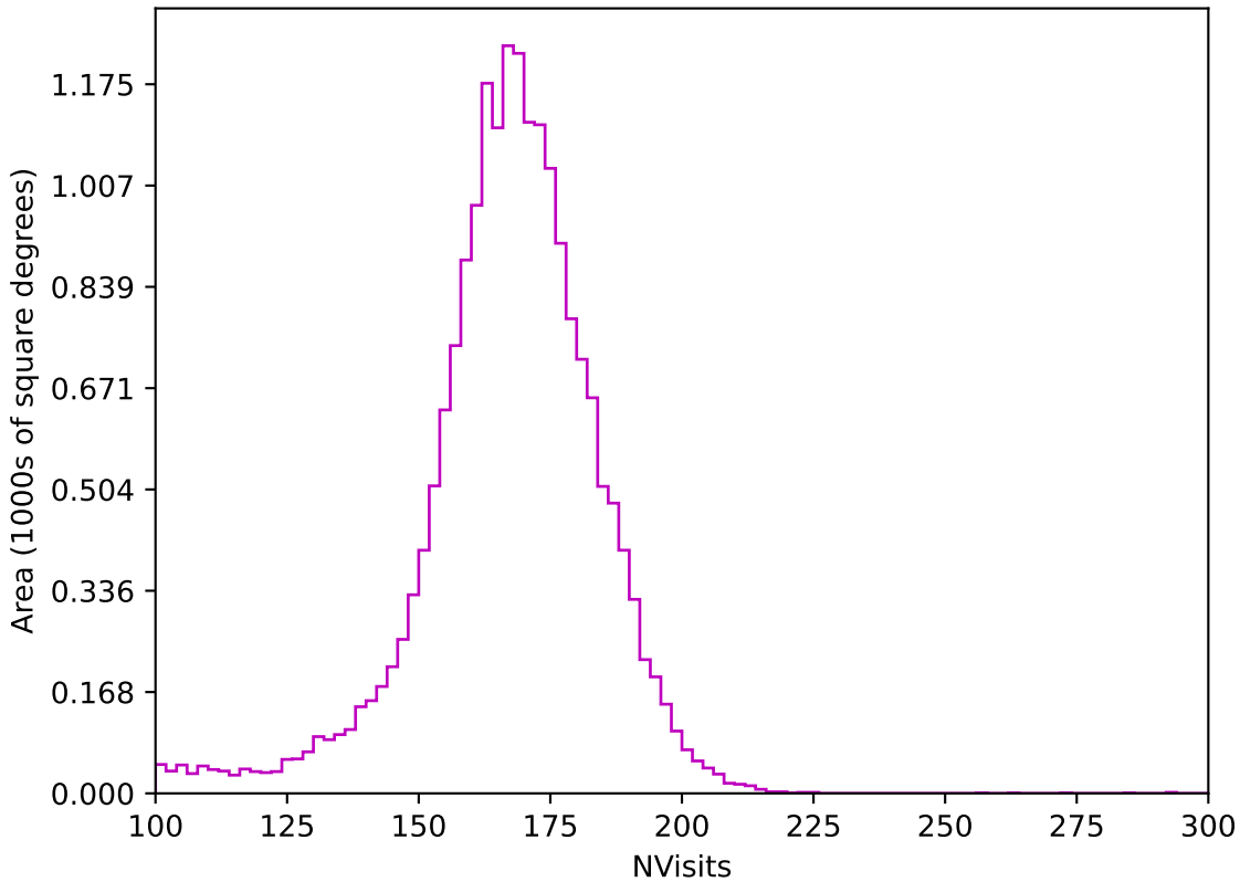
too_elab_r8_d3_gz_v3.4_10yrs All sky z band: NVisits
