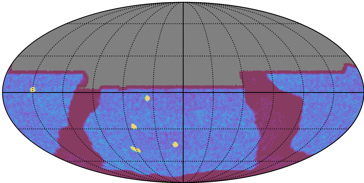
too_elab_r8_d3_gz_v3.4_10yrs All sky y band: NVisits
