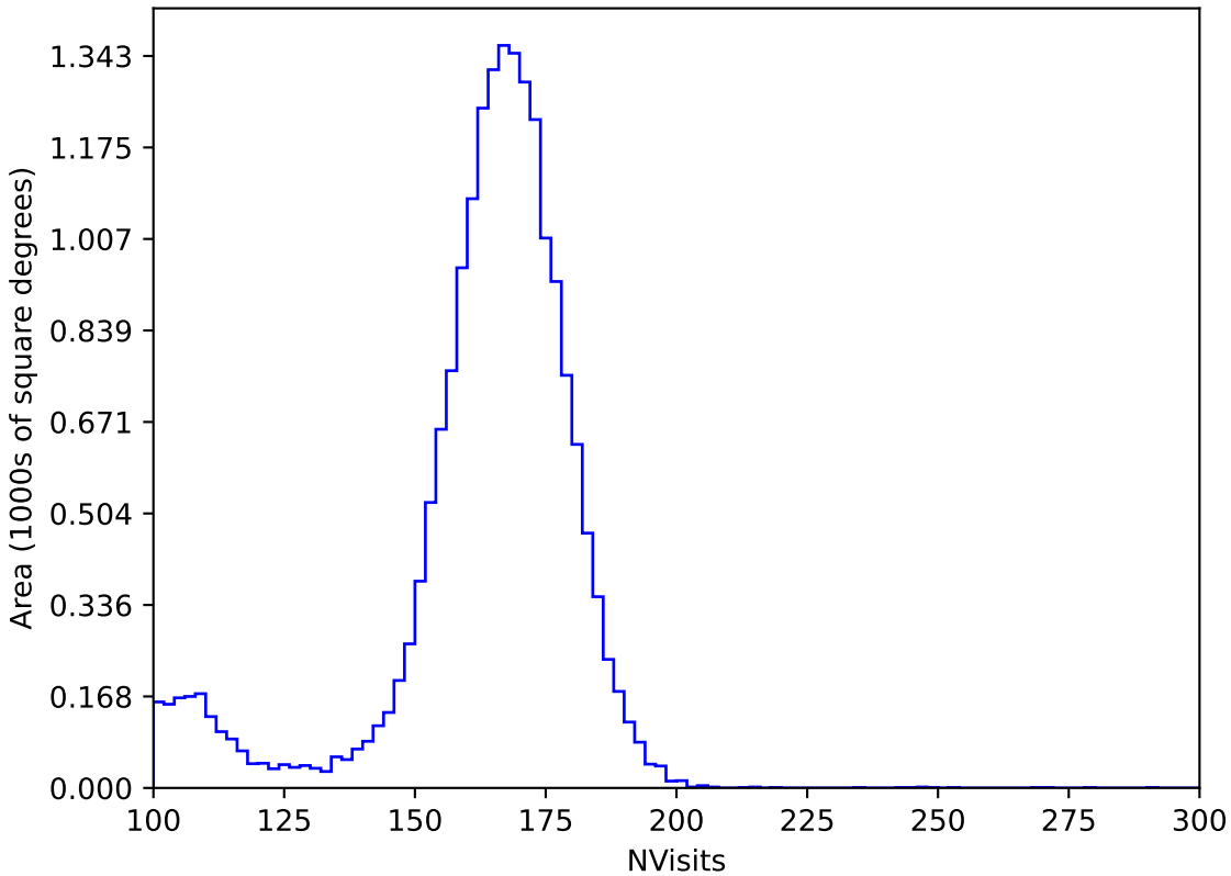
too_elab_r8_d3_gz_v3.4_10yrs All sky y band: NVisits
