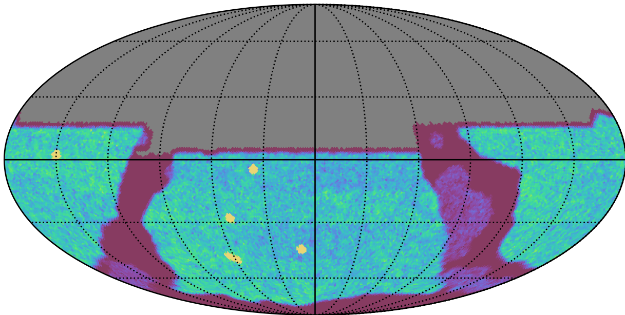
too_elab_r8_d3_gz_v3.4_10yrs All sky u band: NVisits
