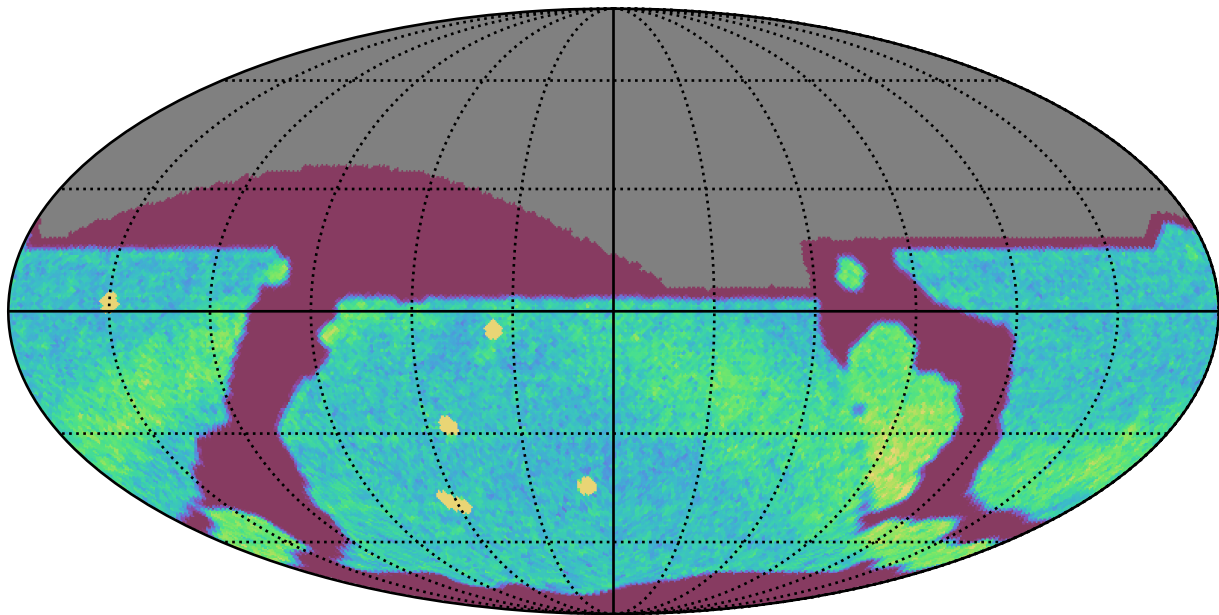
too_elab_r8_d3_gz_v3.4_10yrs All sky r band: NVisits
