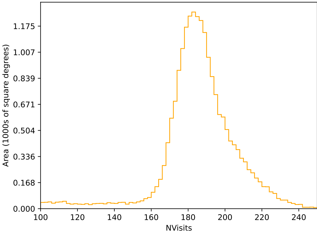
too_elab_r8_d3_gz_v3.4_10yrs All sky r band: NVisits
