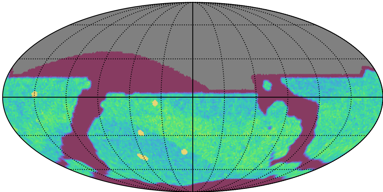
too_elab_r8_d3_gz_v3.4_10yrs All sky i band: NVisits
