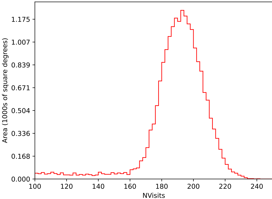
too_elab_r8_d3_gz_v3.4_10yrs All sky i band: NVisits
