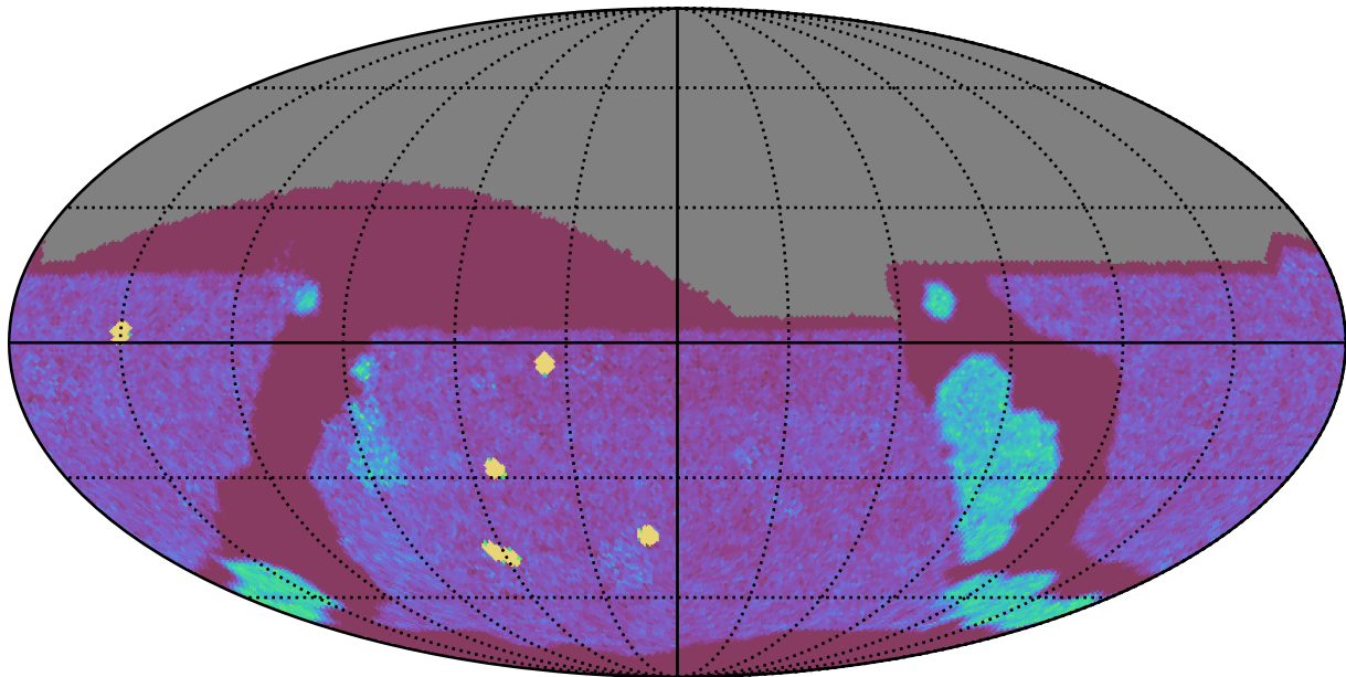
too_elab_r8_d3_gz_v3.4_10yrs All sky g band: NVisits
