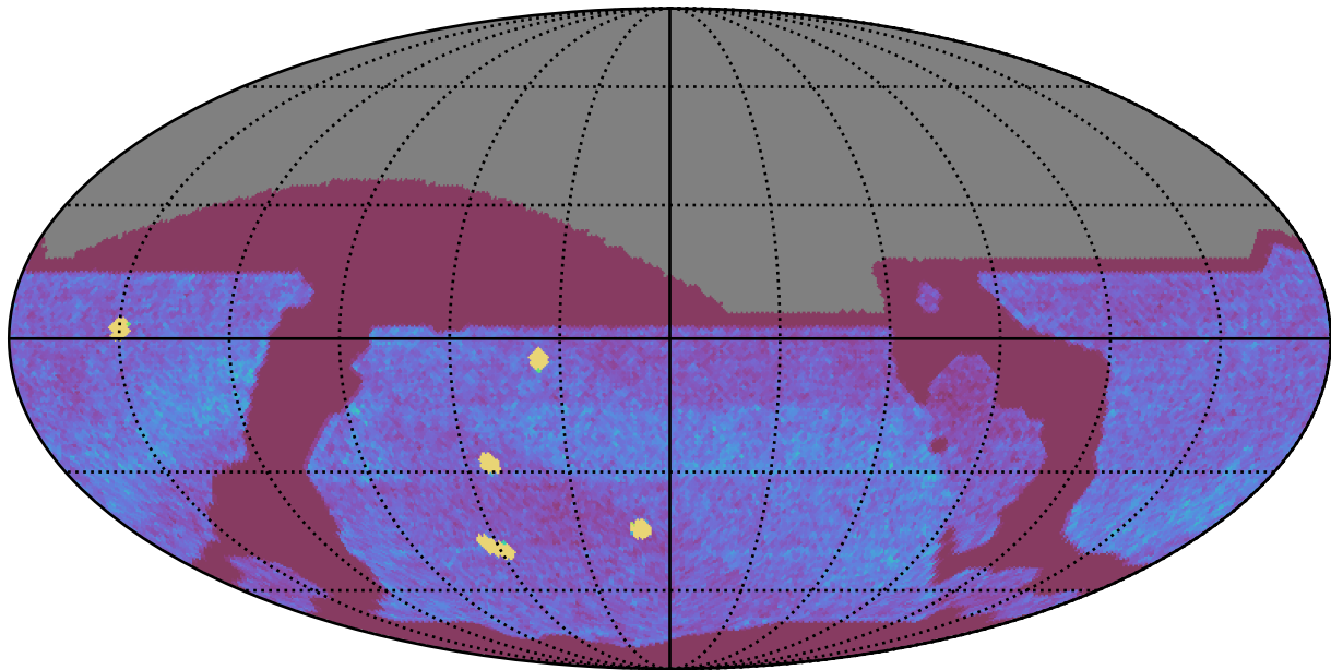
too_elab_r8_d3_gz_v3.4_10yrs All sky all bands: NVisits
