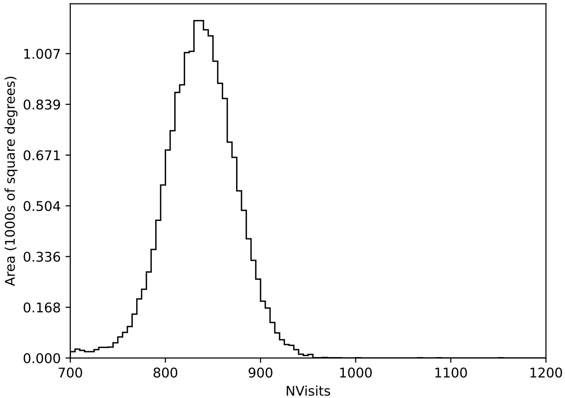
too_elab_r8_d3_gz_v3.4_10yrs All sky all bands: NVisits
