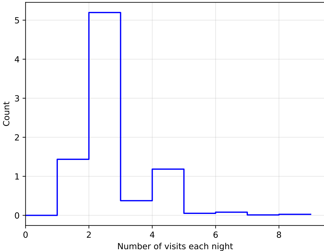
1e6 too_elab_r8_d3_gz_v3.4_10yrs WFD: NVisitsPerNight
