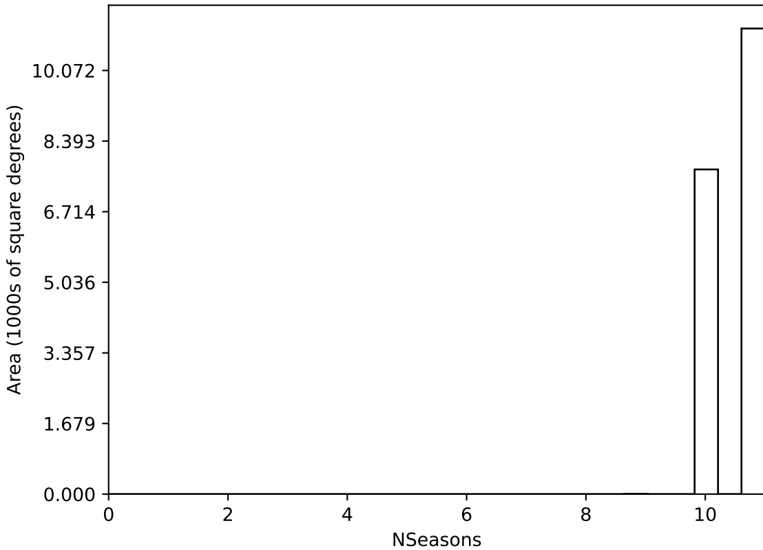
too_elab_r8_d3_gz_v3.4_10yrs WFD all bands: NSeasons
