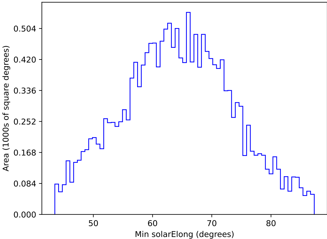
too_elab_r8_d3_gz_v3.4_10yrs WFD y band: Min solarElong
