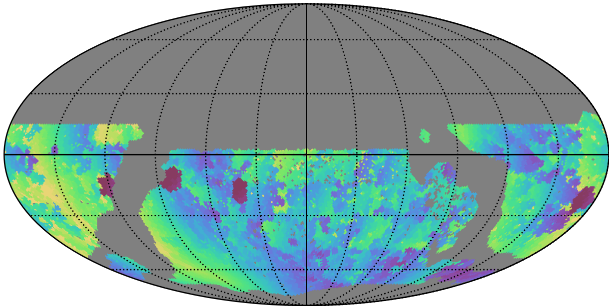
too_elab_r8_d3_gz_v3.4_10yrs WFD g band: Min solarElong
