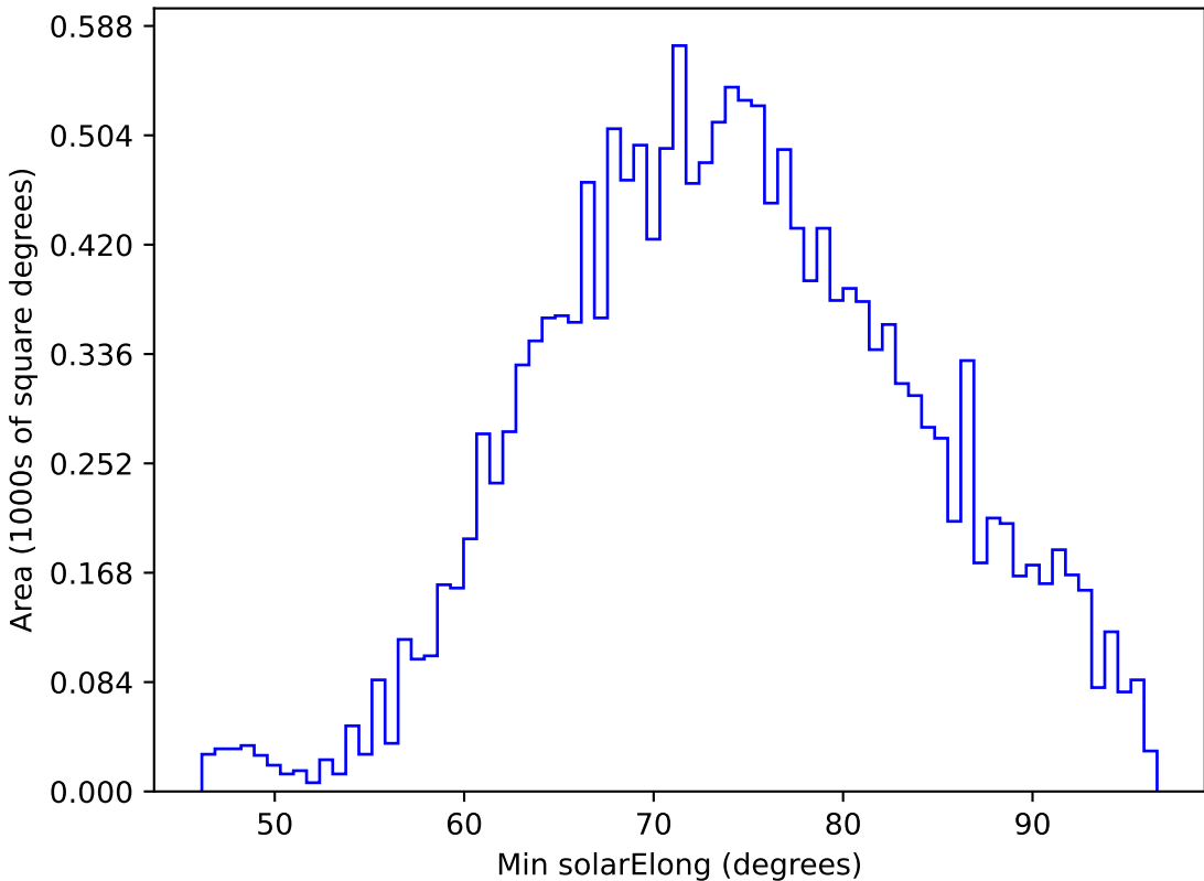
too_elab_r8_d3_gz_v3.4_10yrs WFD g band: Min solarElong
