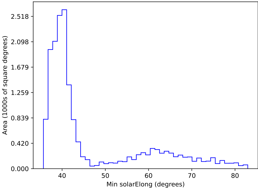
too_elab_r8_d3_gz_v3.4_10yrs WFD all bands: Min solarElong
