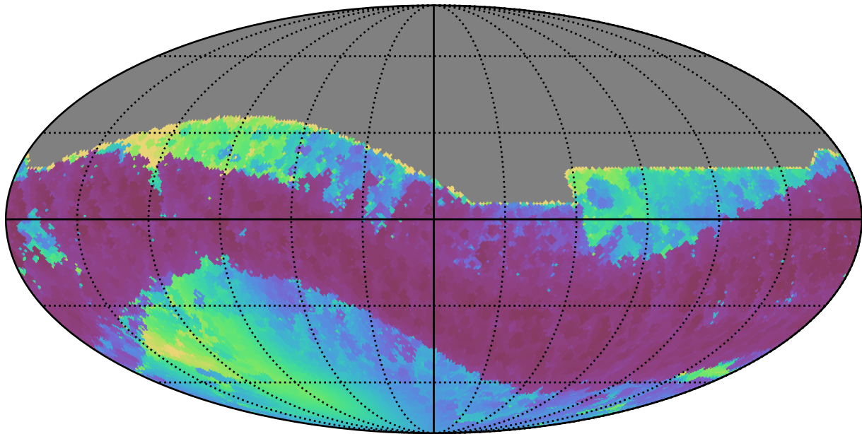
too_elab_r8_d3_gz_v3.4_10yrs All sky z band: Min solarElong
