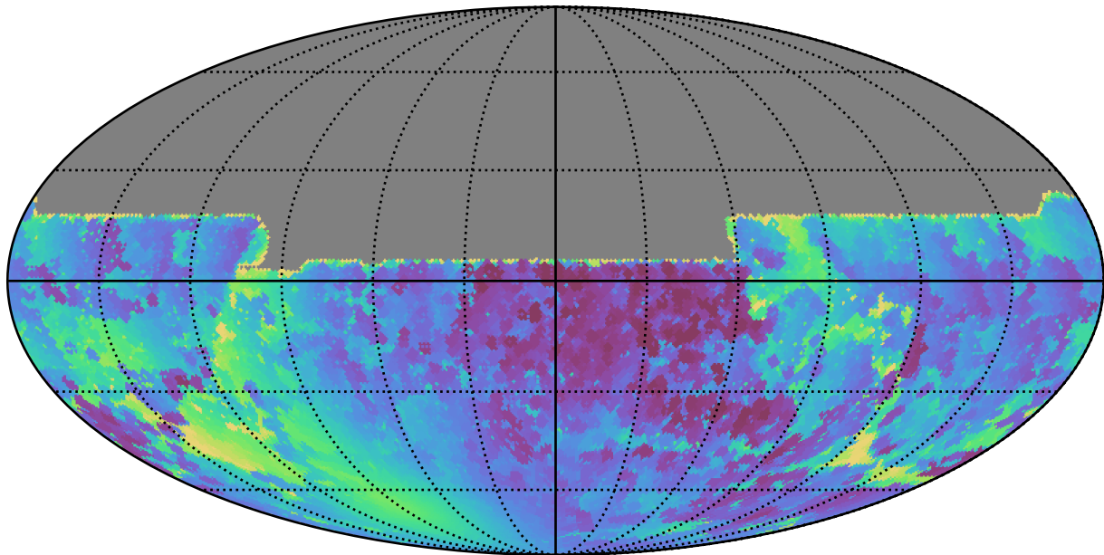
too_elab_r8_d3_gz_v3.4_10yrs All sky y band: Min solarElong
