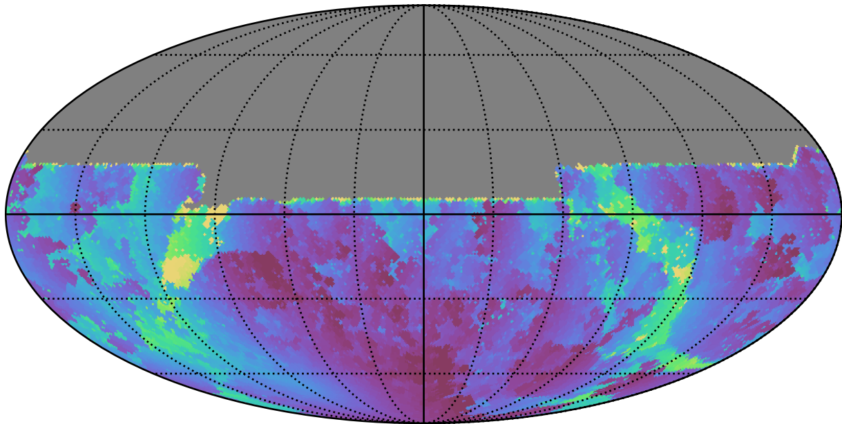
too_elab_r8_d3_gz_v3.4_10yrs All sky u band: Min solarElong
