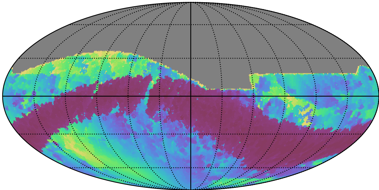
too_elab_r8_d3_gz_v3.4_10yrs All sky r band: Min solarElong
