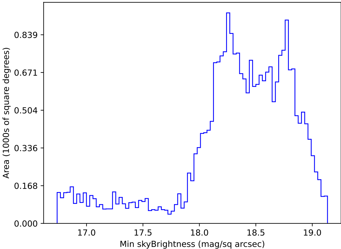
too_elab_r8_d3_gz_v3.4_10yrs Yr 1 z band: Min skyBrightness
