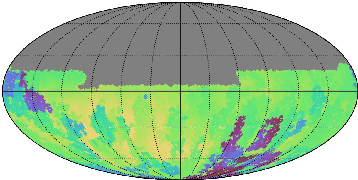
too_elab_r8_d3_gz_v3.4_10yrs Yr 1 u band: Min skyBrightness
