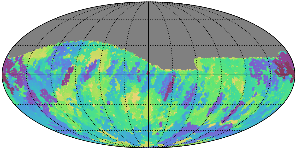
too_elab_r8_d3_gz_v3.4_10yrs Yr 1 r band: Min skyBrightness
