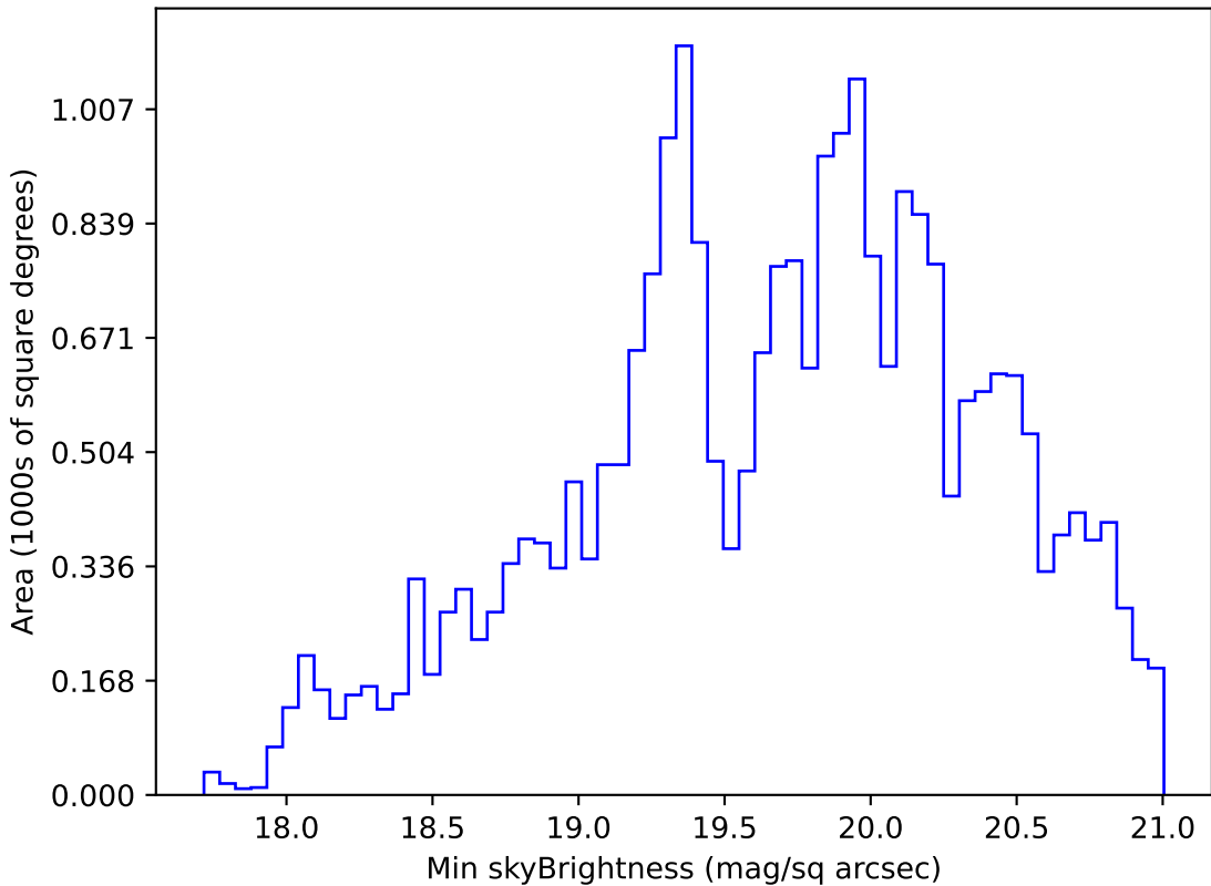
too_elab_r8_d3_gz_v3.4_10yrs Yr 1 r band: Min skyBrightness
