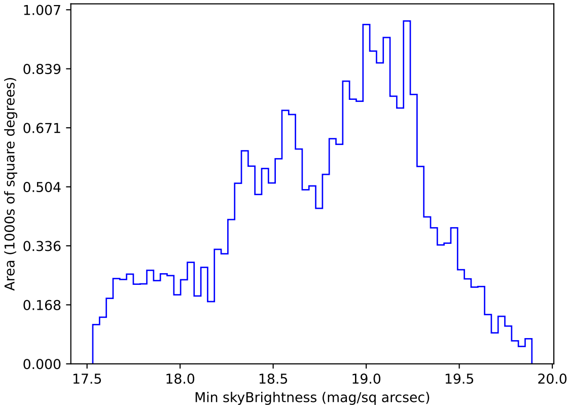
too_elab_r8_d3_gz_v3.4_10yrs Yr 1 i band: Min skyBrightness
