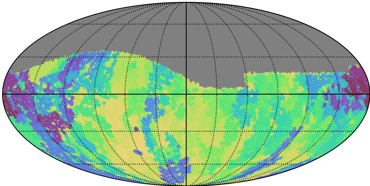
too_elab_r8_d3_gz_v3.4_10yrs Yr 1 g band: Min skyBrightness
