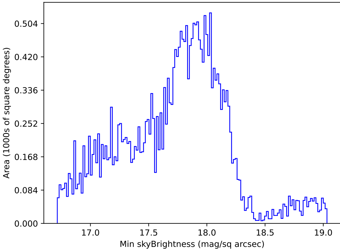
too_elab_r8_d3_gz_v3.4_10yrs Yr 1 all bands: Min skyBrightness
