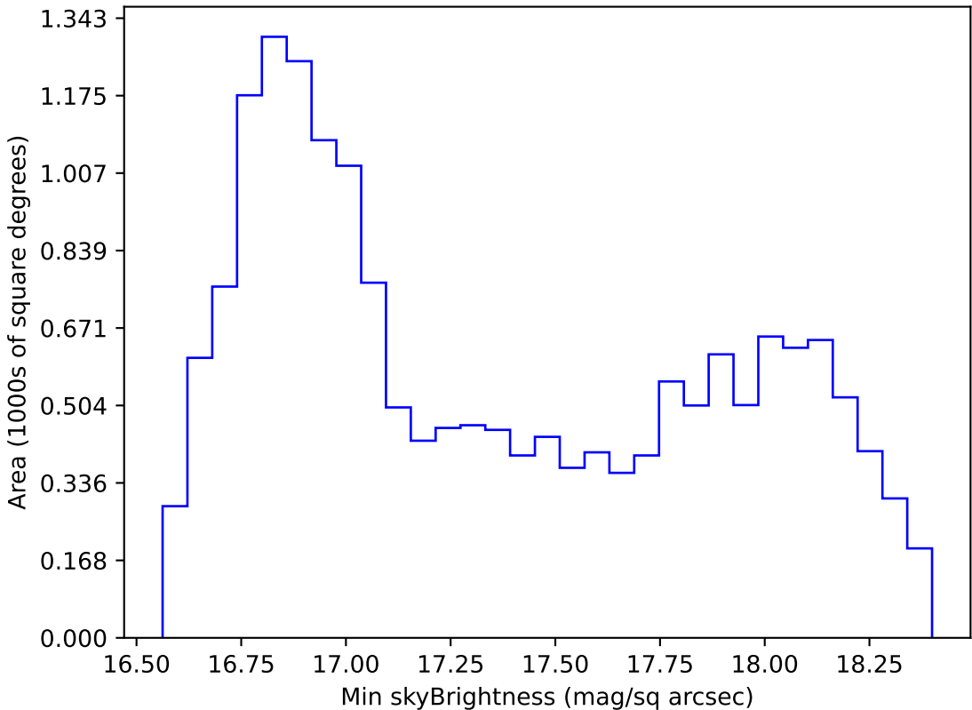
too_elab_r8_d3_gz_v3.4_10yrs WFD z band: Min skyBrightness
