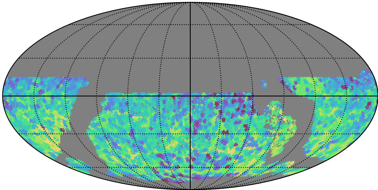
too_elab_r8_d3_gz_v3.4_10yrs WFD y band: Min skyBrightness
