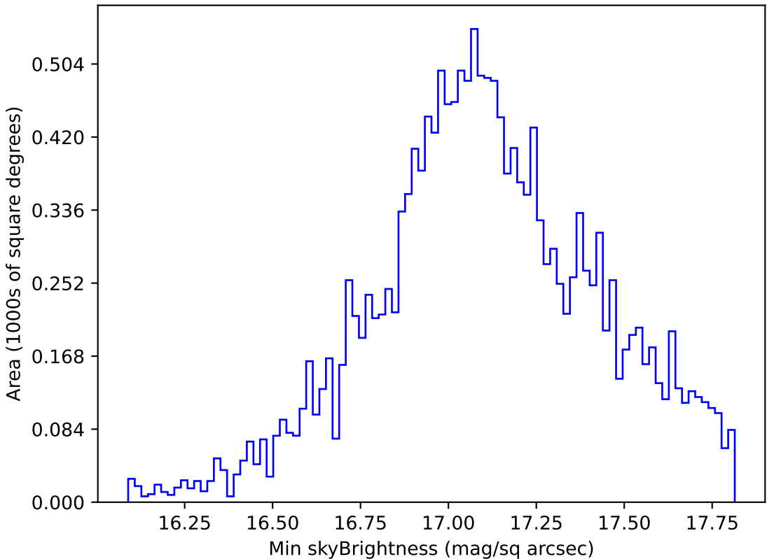
too_elab_r8_d3_gz_v3.4_10yrs WFD y band: Min skyBrightness
