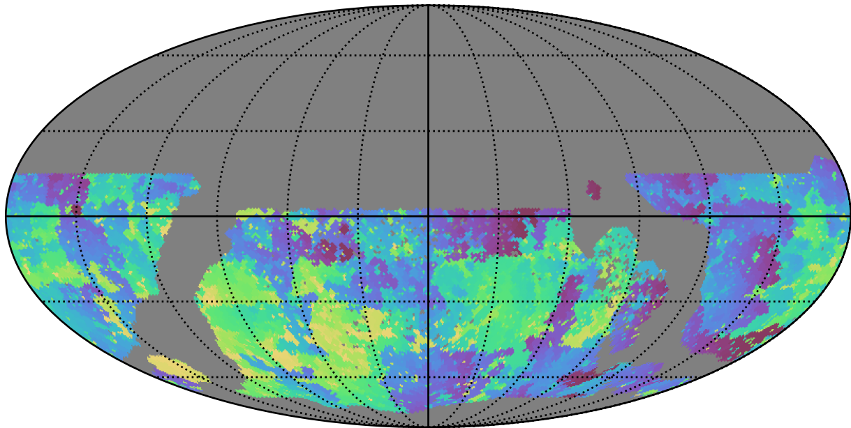
too_elab_r8_d3_gz_v3.4_10yrs WFD u band: Min skyBrightness
