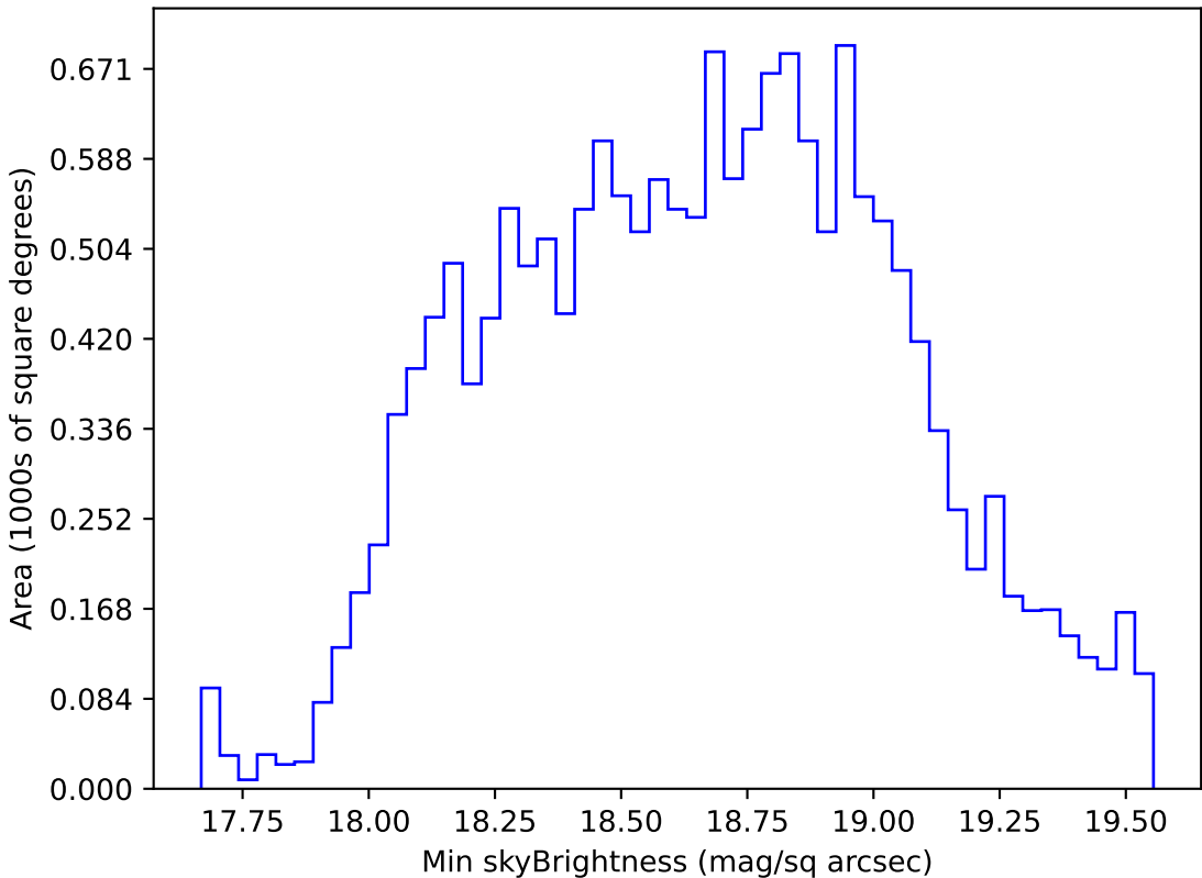
too_elab_r8_d3_gz_v3.4_10yrs WFD r band: Min skyBrightness
