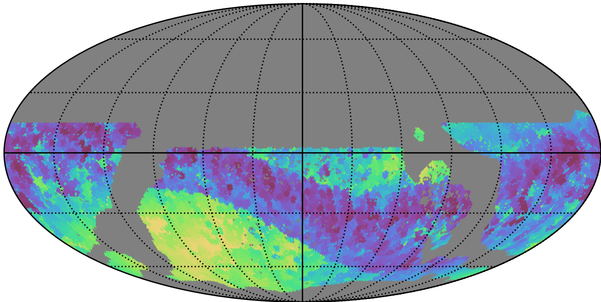
too_elab_r8_d3_gz_v3.4_10yrs WFD i band: Min skyBrightness
