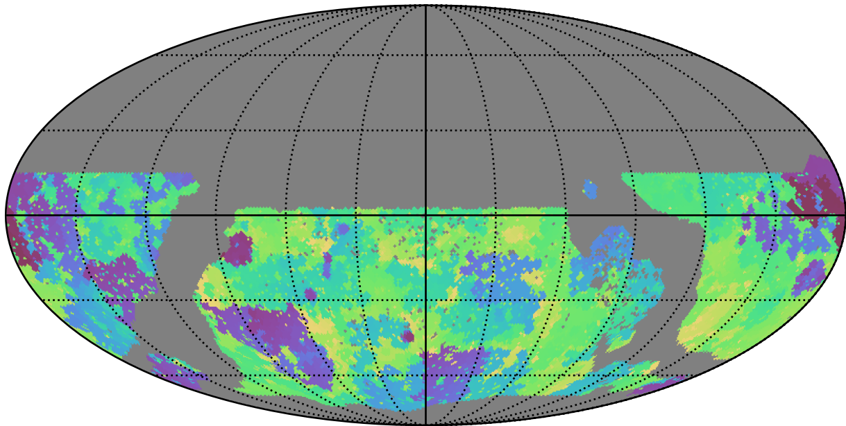
too_elab_r8_d3_gz_v3.4_10yrs WFD g band: Min skyBrightness
