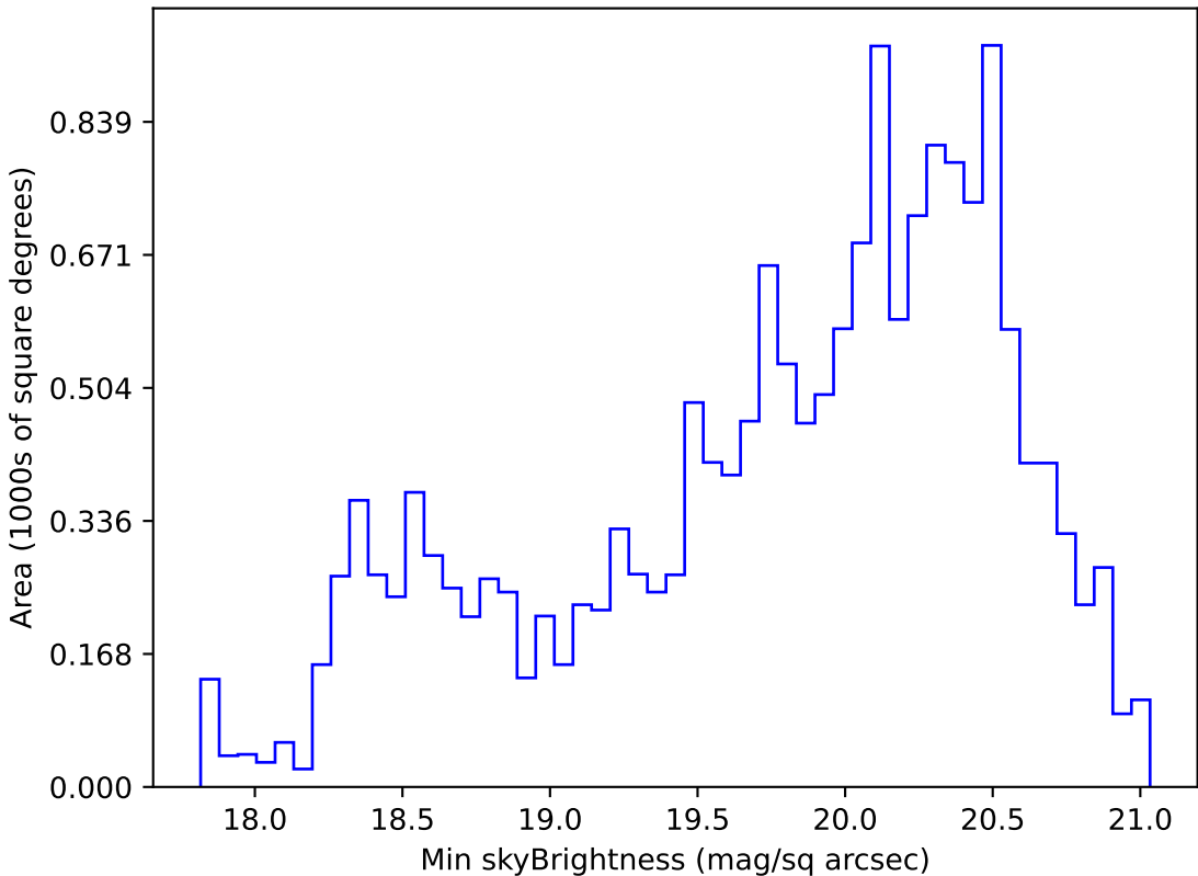
too_elab_r8_d3_gz_v3.4_10yrs WFD g band: Min skyBrightness
