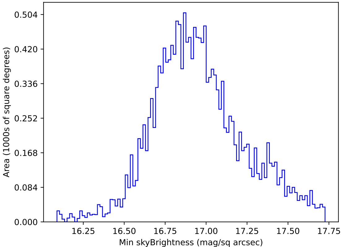
too_elab_r8_d3_gz_v3.4_10yrs WFD all bands: Min skyBrightness
