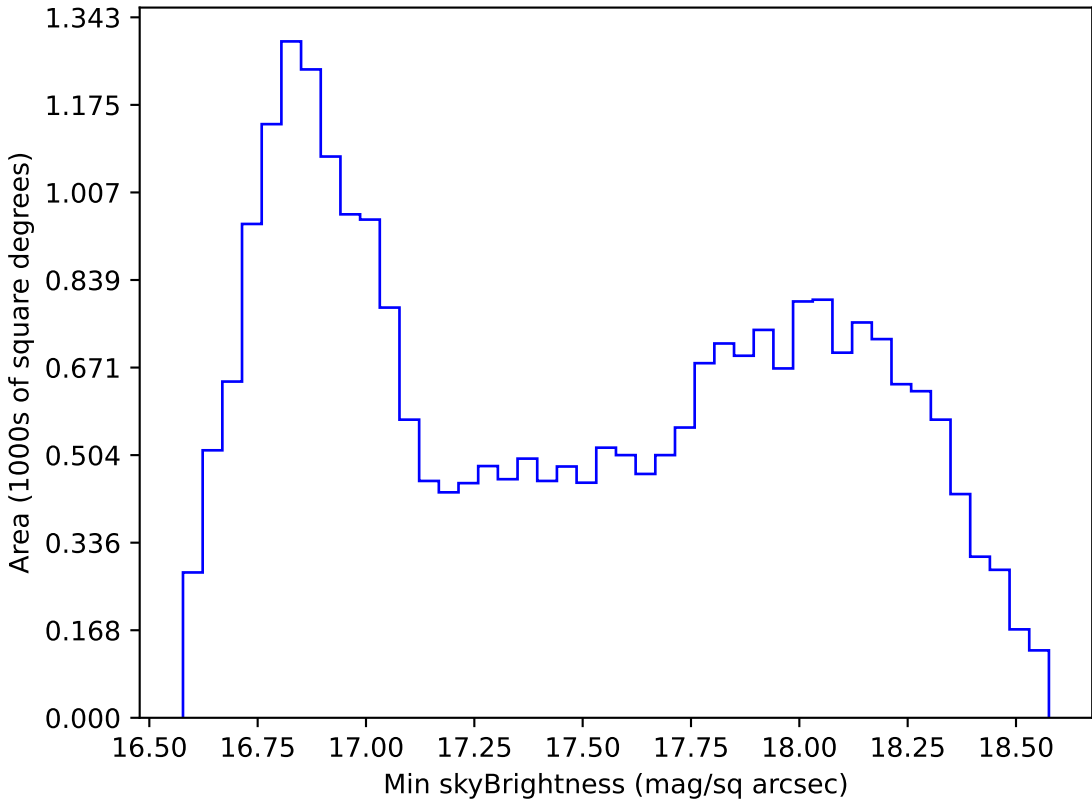
too_elab_r8_d3_gz_v3.4_10yrs All sky z band: Min skyBrightness
