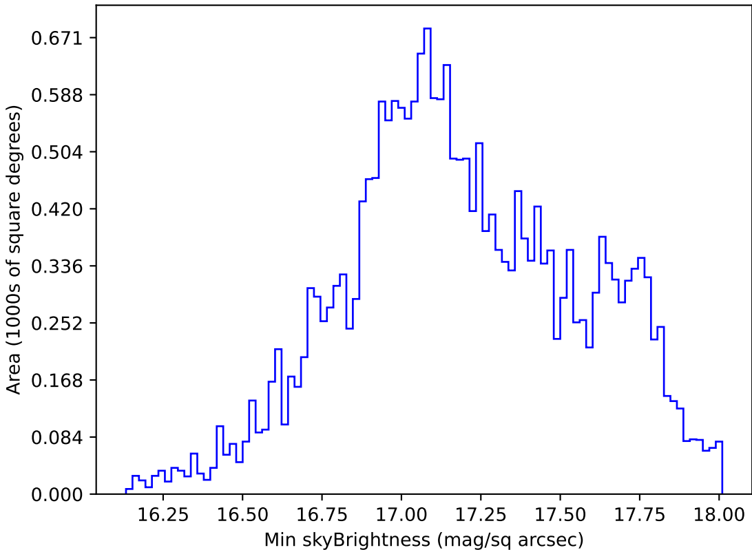
too_elab_r8_d3_gz_v3.4_10yrs All sky y band: Min skyBrightness
