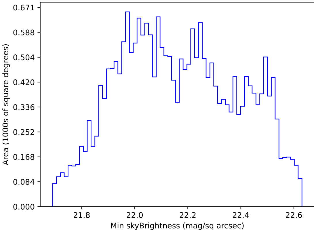
too_elab_r8_d3_gz_v3.4_10yrs All sky u band: Min skyBrightness
